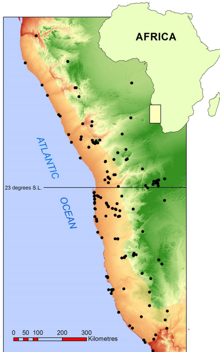
The Namib Desert forms a continuous strip 100-150km wide between the Atlantic coast and the escarpment. Here, the desert is shown in light brown, with the escarpment zone in shades of green. During the Last Glacial Maximum, ending approximately 10 000 years ago, the coastline lay up to 100km further west and the desert extended at least 400km into the interior. The black dots are dated archaeological sites.
